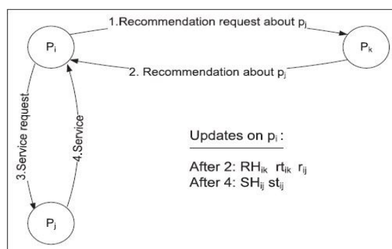
Fig.4 Operations when receiving a recommendation and having an interaction.
